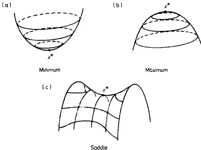
Figure 2.1.3 Types of stationary point
