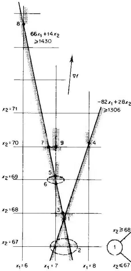
Figure 13.1.3 Solution of (13.1.5) by the branch and bound method
