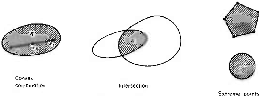
Figure 9.4.1 Convex sets
