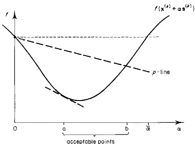
Figure 2.5.2 Wolfe–Powell conditions
