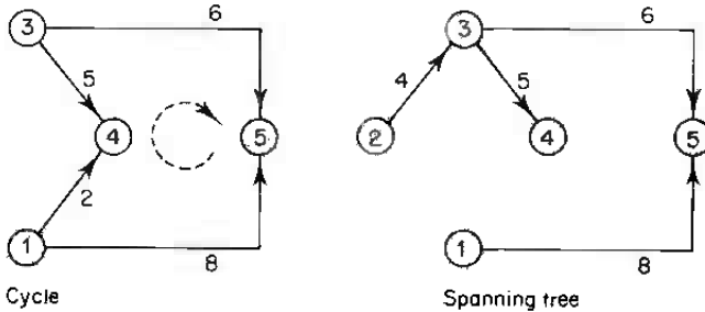
Figure 13.3.1 Graph theory concepts
