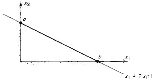
Figure 8.1.1 Constraints for a simple LP problem
