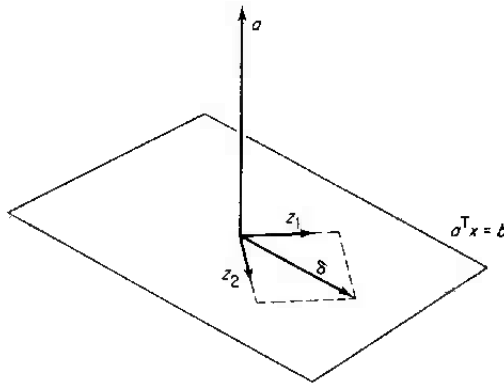
Figure 10.1.1 Reduced coordinates for the feasible region
