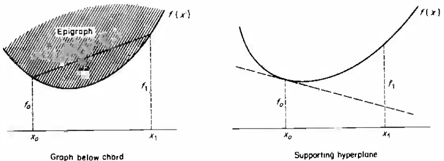
Figure 9.4.2 Convex functions
