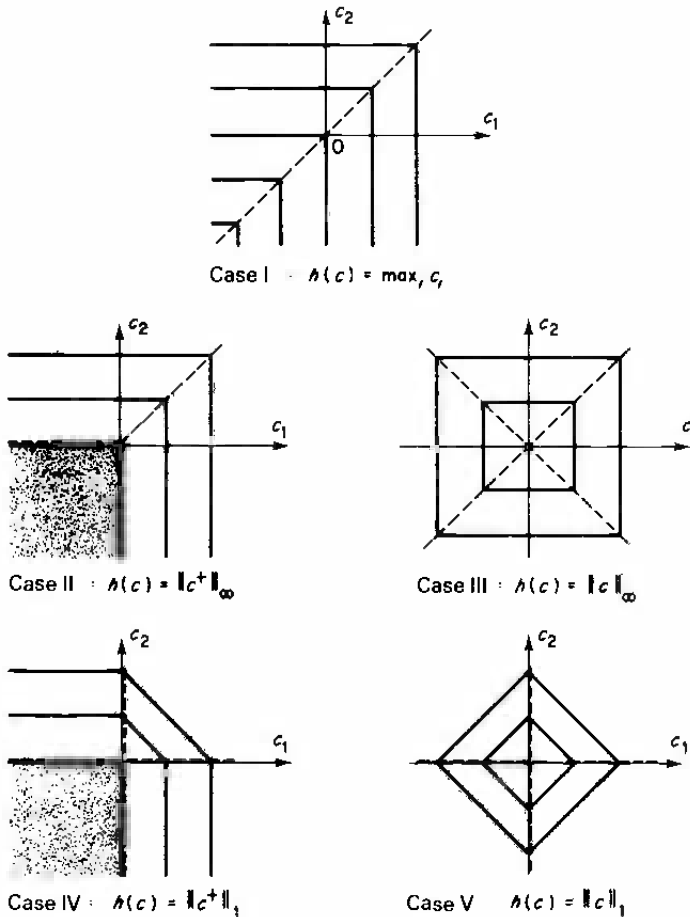
Figure 14.1.2 Contours of polyhedral convex functions
