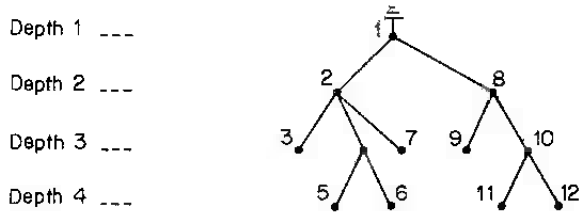
Figure 13.3.4 Depth-first ordering in rooted spanning tree
