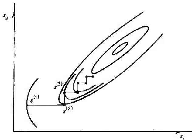
Figure 2.2.3 The method of alternating variables
