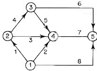
Connected graph with 5 nodes and 8 arcs
