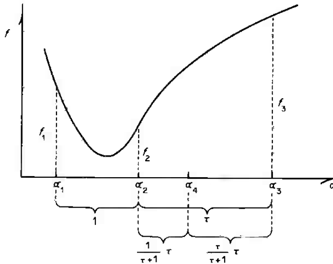
Figure 2.6.1 Golden section search
