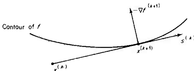
Figure 2.3.1 The exact line search
