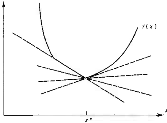
Figure 14.2.1 Supporting hyperplanes to a non-smooth convex function
