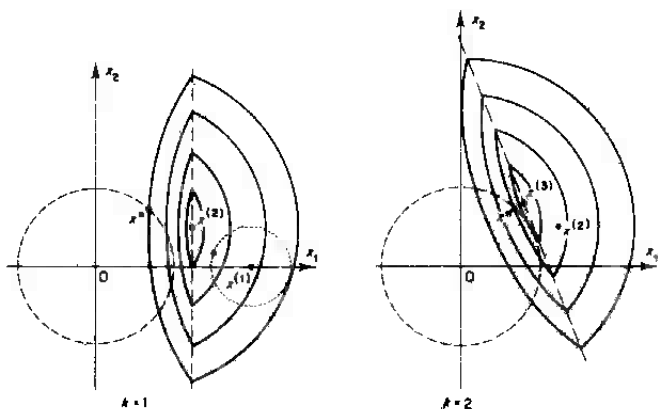
Figure 14.4.4 Contours of the approximating function in the SNQP method
