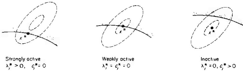
Figure 9.1.2 Complementarity
