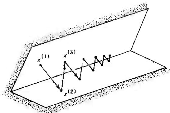
Figure 11.3.1 Zigzagging
