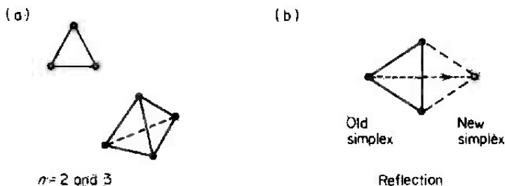
Figure 2.2.1 Regular simplices
