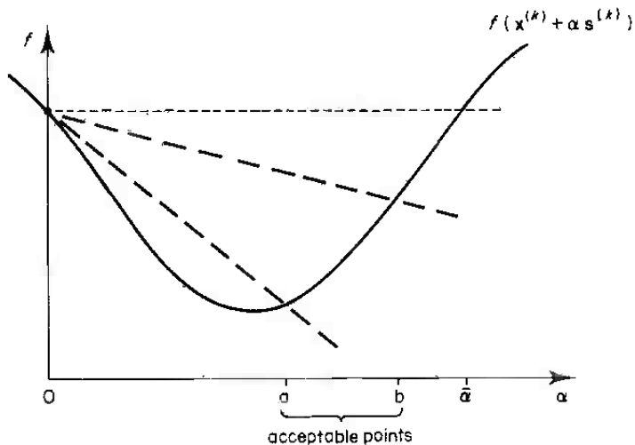
Figure 2.5.1 Goldstein conditions
