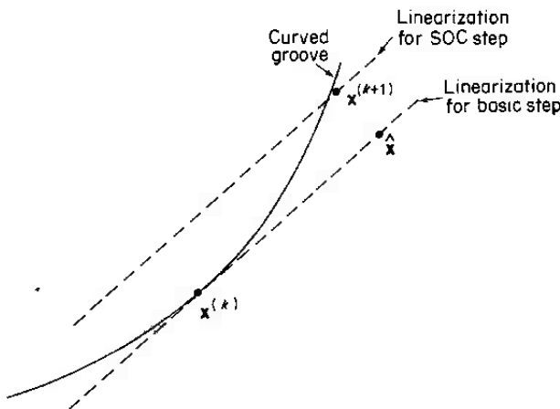
Figure 14.4.6 The second order correction step
