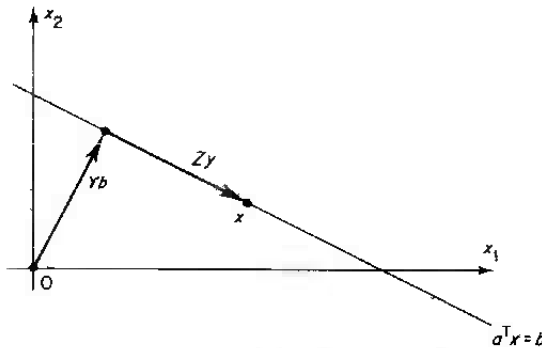
Figure 10.1.2 Generalized elimination in the special case (10.1.18)
