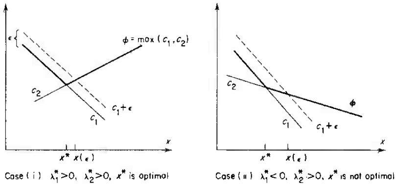
Figure 14.1.3. Interpretation of multipliers in NSO
