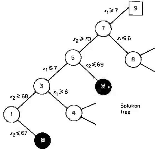
Figure 13.1.3 Solution of (13.1.5) by the branch and bound method
