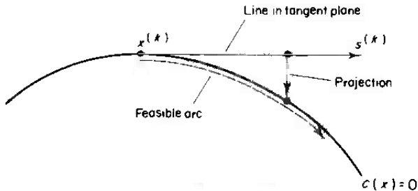
Figure 12.5.1 Feasible direction search
