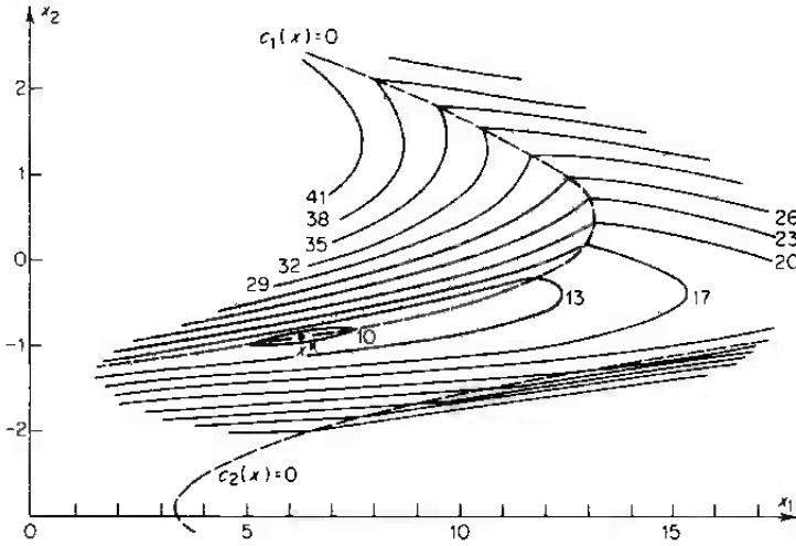
Figure 14.2.3 Contours for the scaled L_1 Freudenstein and Roth problem, Question 14.9
