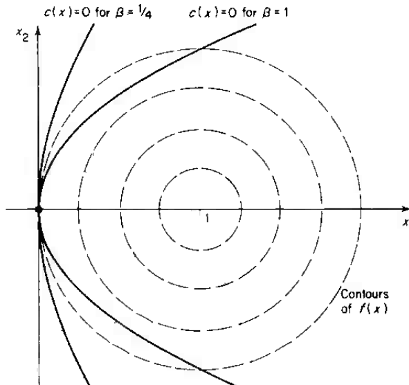
Figure 9.3.1 Second order conditions
