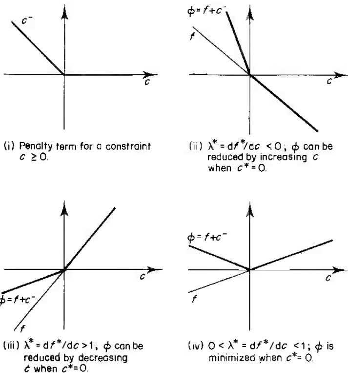
Figure 12.3.2 Optimality conditions for an L_1 exact penalty function
