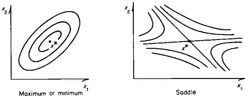
Figure 2.1.4 Contours for stationary points
