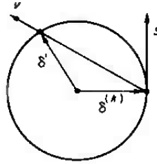
Figure 5.2.1 Construction of the vector \delta'
