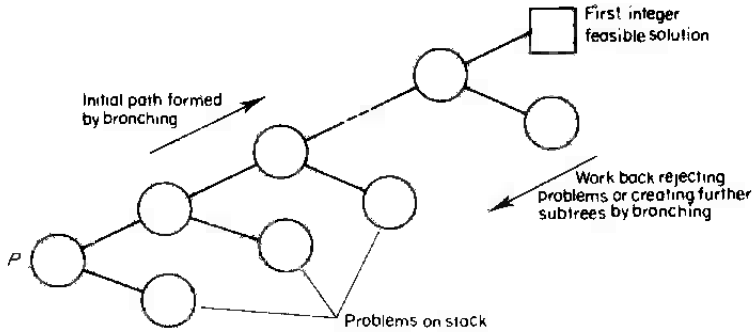
Figure 13.1.2 Progress of the stack method
