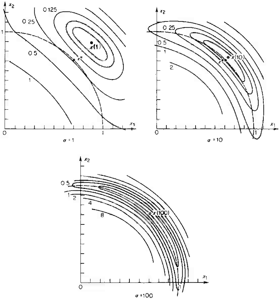
Figure 12.1.2 Increasing ill-conditioning in penalty functions (contours of \phi - \phi_{\min} in powers of 2)
