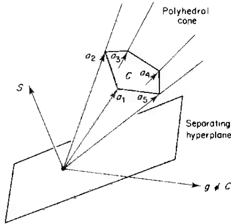
Figure 9.2.2 Existence of a separating hyperplane
