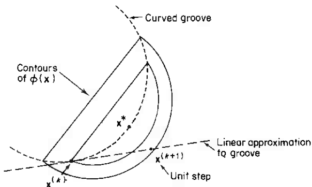
Figure 14.4.5 Maratos effect
